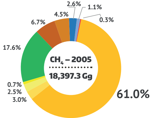
FIGURE 2.4 Share of CH 4 emissions (2005)
