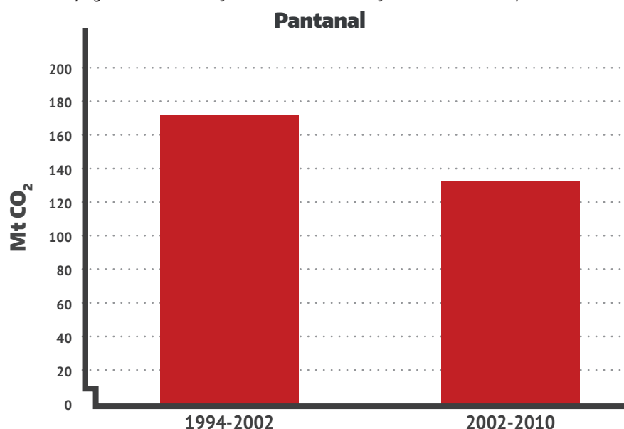
FIGURE 3.10 Net anthropogenic emissions of the Pantanal biome for the considered periods
