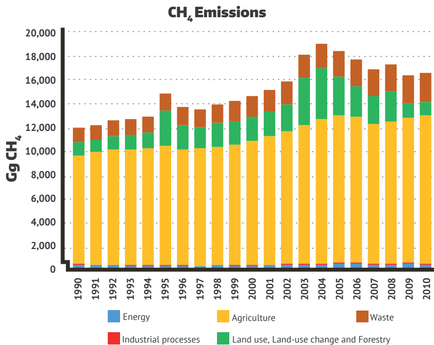
FIGURE 2.6 Evolution of CH 4 emissions
