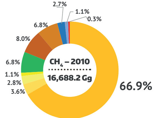
FIGURE 2.5 Share of CH 4 emissions (2010)
